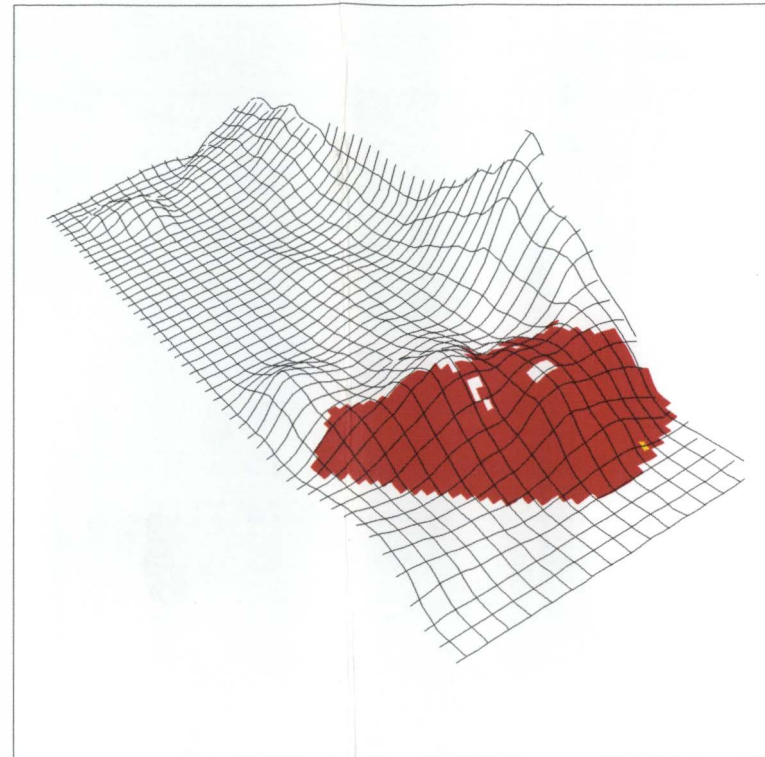
Simulated fire shape after 30 minutes
