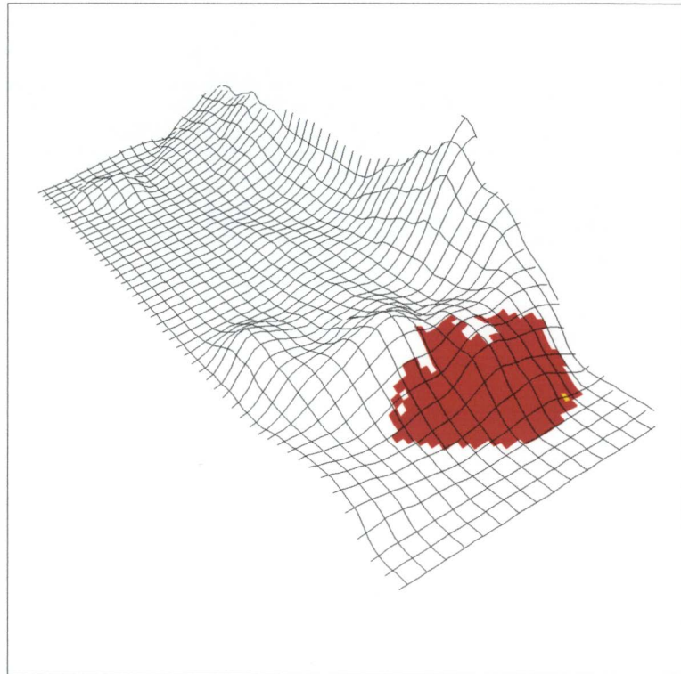
Simulated fire shape after 15 minutes
