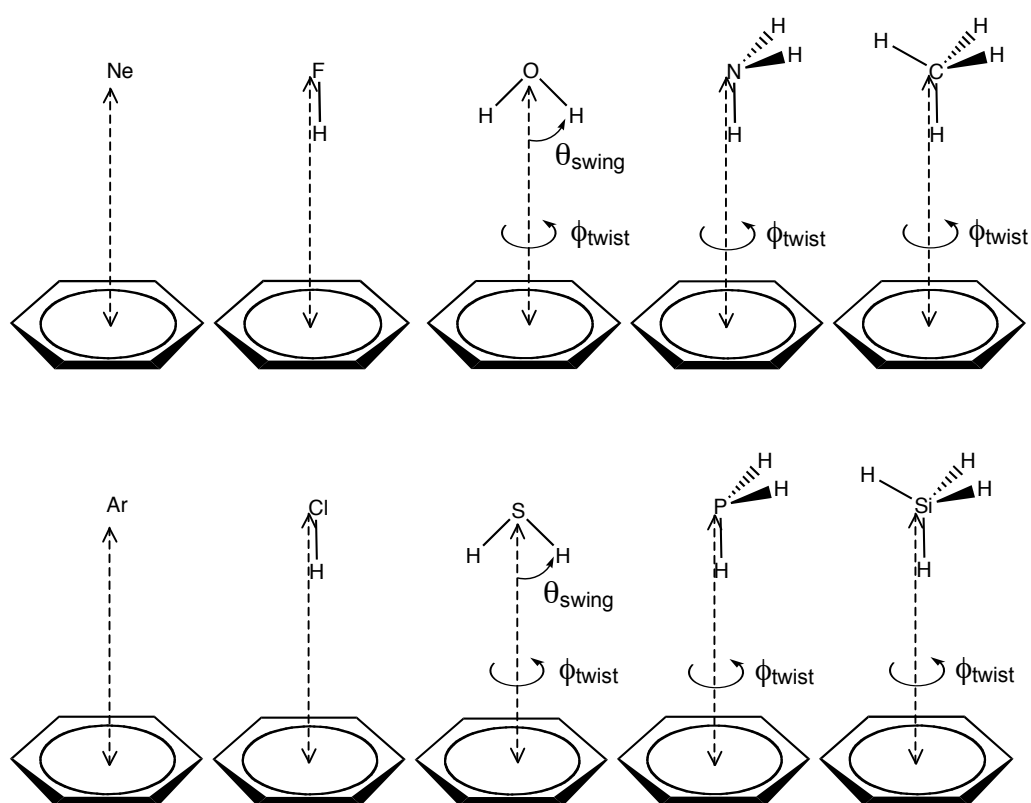
Figure 1. Initial conformations of all benzene : small molecule complexes.
