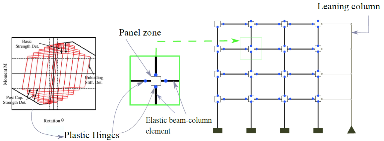
Fig. 7 – Schematic of the four-storey steel moment frame building model, and the modified IMK bilinear hysteretic model used for plastic hinges.
