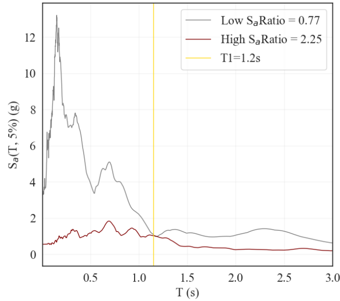
Fig. 1 – Response spectra of two ground motions scaled to a common value of S_a(1.2s) = 1g with low and high S_aRatio(1.2s, 0.2s, 3.6s) values.
