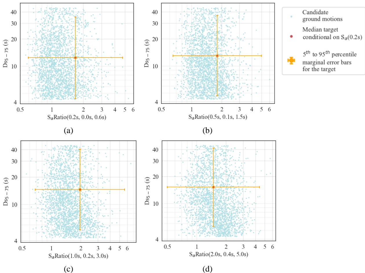
Fig. 3 – Candidate ground motions and the distributions of the S_a Ratio and D_{S5-75} targets conditional on the *% exceedance probability of S_a at (a) 0.2 s, (b) 0.5 s, (c) 1.0 s, and (d) 2.0 s
