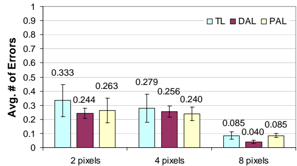
Figure 18: Average # of errors (+/- SE) per size and technique.
