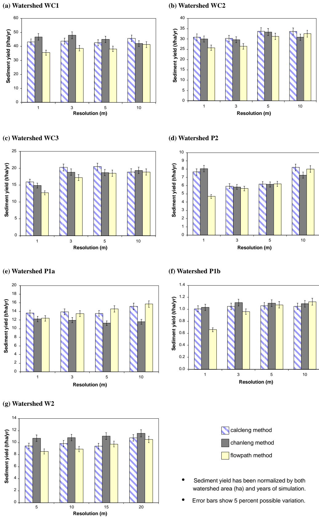
Figure 5. Average hillslope sediment yields with three different methods and four different resolutions.
