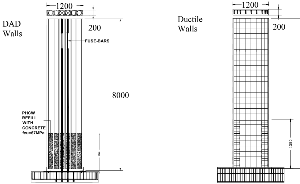
(a) Prototype models of walls for the dynamic analysis.
