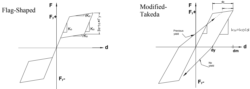
(c) Nonlinear models used for the dynamic analysis of walls.
