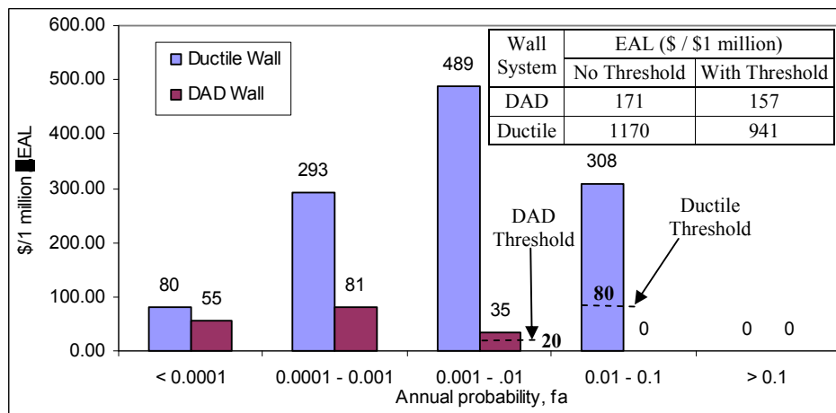
Figure 6(c) Annual financial risk due to earthquakes of different probability
