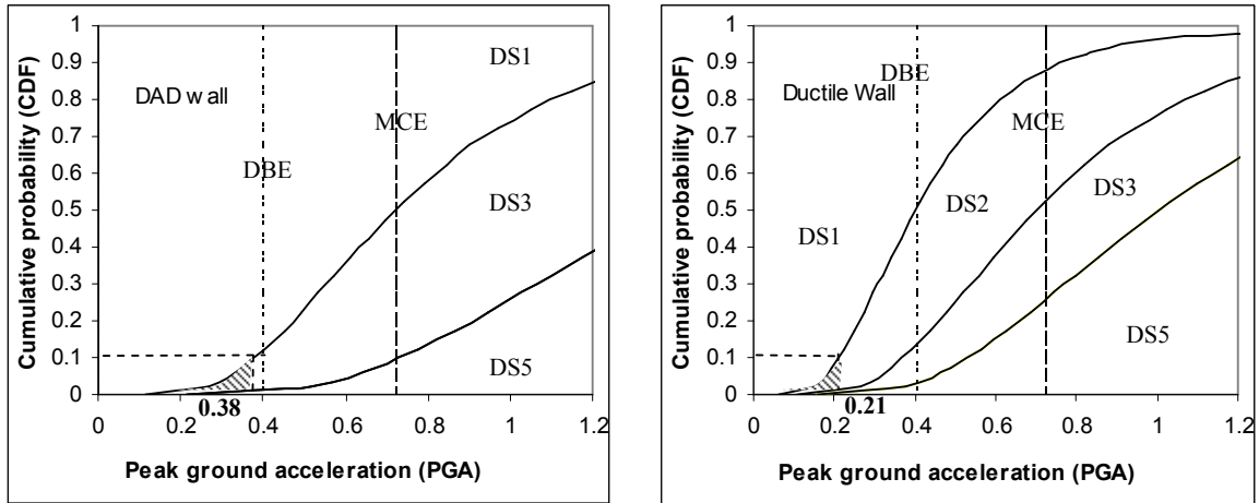
Figure 5(a) Fragility curves for the wall systems.
