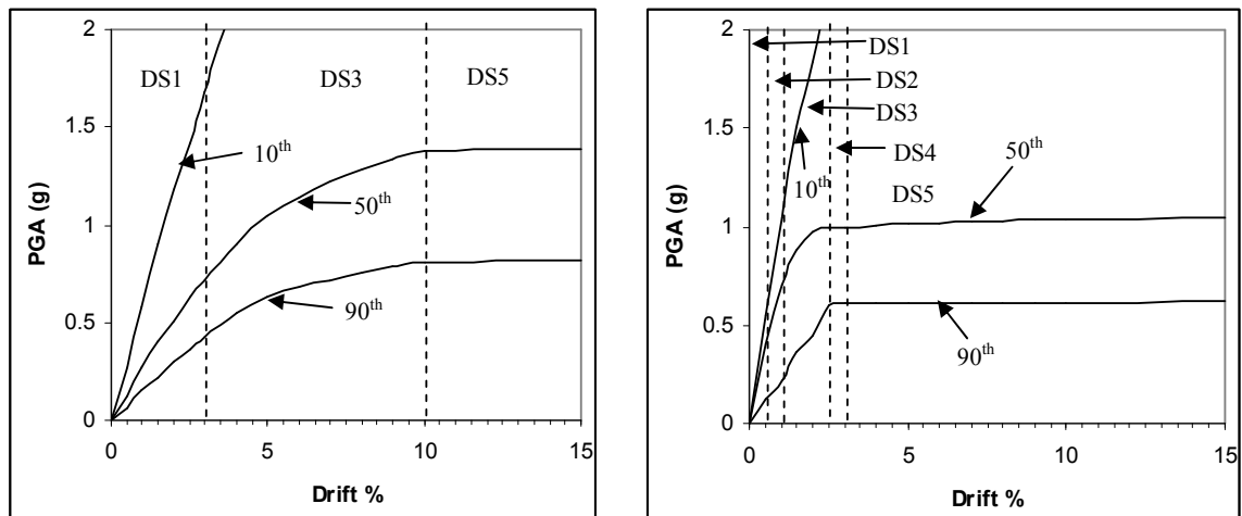
(b) Fitted IDA curves for different percentile response demand with damage states
