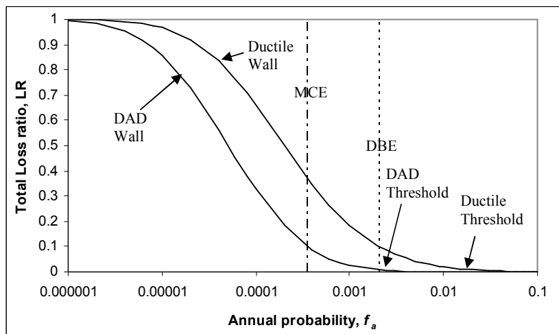
Figure 6(b) Economic Hazard Curves.
