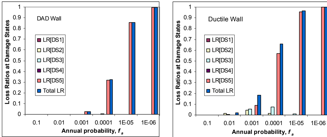
Figure 6(a) Loss ratios inflicted by different damage states to the two wall systems.
