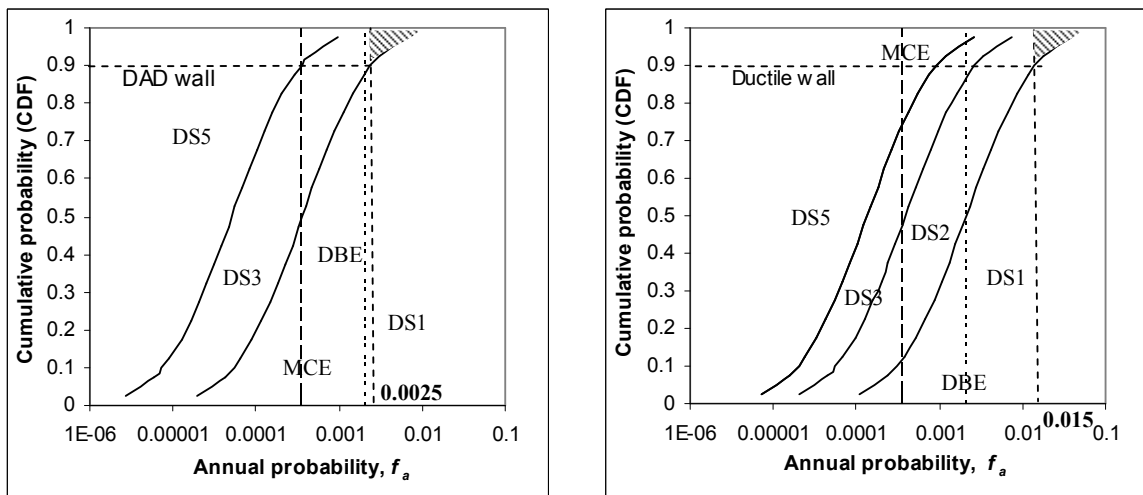
Figure 5(c) Hazard-Survival curves for the two wall systems.
