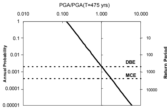
Figure 5(b) Hazard Recurrence Relation (between PGA ( a_g ) and annual probability ( f_a ))
