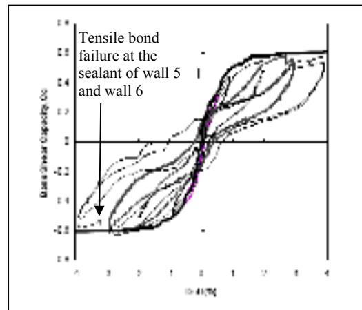
(b) The overall hysteretic performance up to 4% drift of multi-panel super assembly.
