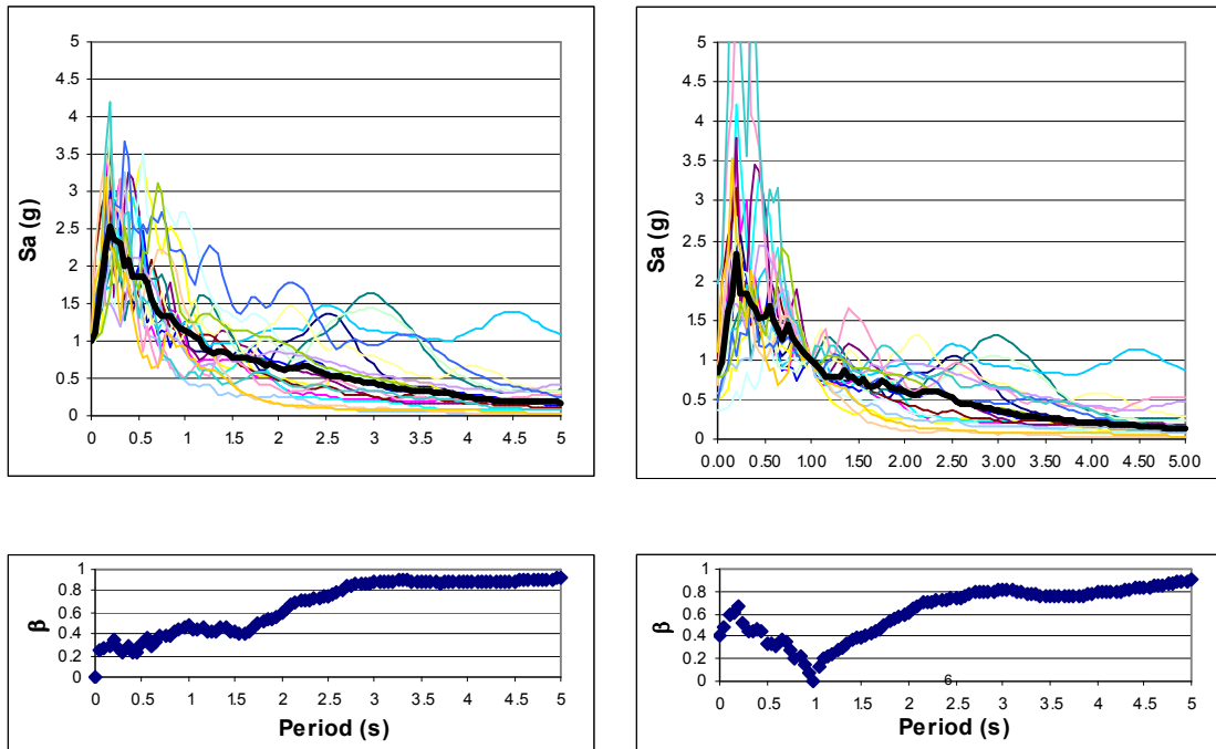
(b) Scaled to a common IM of PGA (1.0g) (c) Scaled to a common IM of S_a(T_n=1\text{sec}, 5\%)
