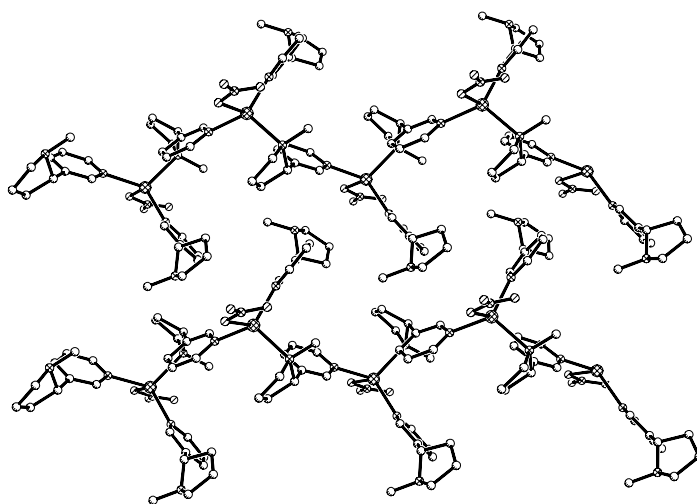
Figure 4. Perspective view, down the a axis, of the extended structure of 3 . Hydrogen atoms are omitted for clarity.
