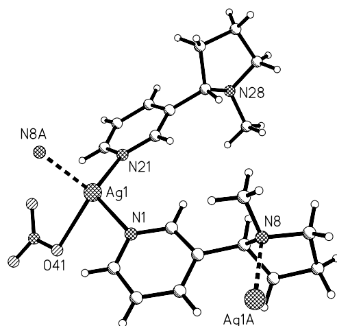
Figure 3. Perspective view of the contents of the asymmetric unit, and attached atoms, in the X-ray structure of 3 . Selected bond lengths (Å) and angles (°): Ag1-N1 2.323(2); Ag1-N8A 2.405(2); Ag1-N21 2.298(2); Ag1-O41 2.500(2); N1-Ag1-N8A 117.93(7); N1-Ag1-N21 120.14(8); N1-Ag1-O41 91.01(7); N8A-Ag1-N21 106.76(8); N8A-Ag1-O41 103.19(7); N21-Ag1-O41 116.05(8).
