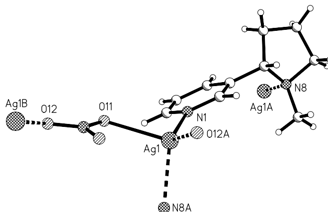
Figure 1. Perspective view of the contents of the asymmetric unit, and attached atoms, in the X-ray structure of 2 . Selected bond lengths (Å) and angles (°): Ag1-N1 2.3007(19); Ag1-N8A 2.3806(17); Ag1-O11 2.5789(19); Ag1-O12A 2.4509(18); N1-Ag1-N8A 125.35(6); N1-Ag1-O11 85.22(6); N1-Ag1-O12A 127.86(7); N8A-Ag1-O11 102.81(7); N8A-Ag1-O12A 92.48(7); O11-Ag1-O12A 123.47(7).
