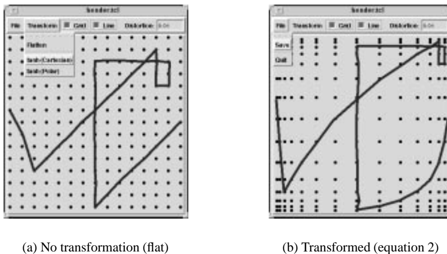
Figure 1: Experimenting with fisheye transformations
