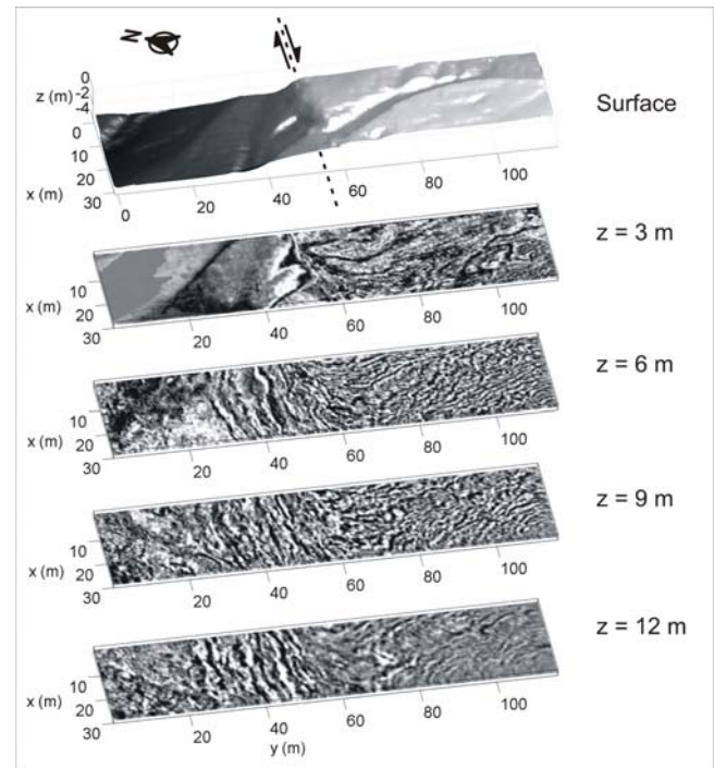
Figure 3. (a) Illuminated perspective view of topography over the 3-D GPR volume. The dashed line and arrows indicate the fault's mapped location and sense of motion. (b) to (e) Depth converted time slices extracted from the migrated GPR volume at z = 3 m, 6 m, 9 m and 12 m.
