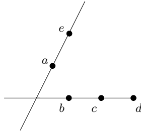
FIGURE 1. A non-trivial 2-separation of a partitioned matroid.
