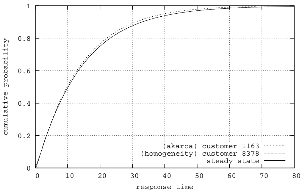
Figure 5.26: F_{R_i}(x) at the average truncation points ( \bar{l}_E = \{283, 1163\} ; \bar{l}_F = \{54, 8378\} ) of the M/E_2/1 queue compared with the steady state distribution F_{R_\infty}(x) at different traffic loads \rho .
