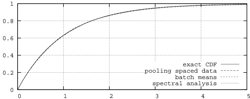
Figure 6.9: Exact and estimated CDFs of basic processes with negative exponential distribution: \text{Exp}(x; 1) .
