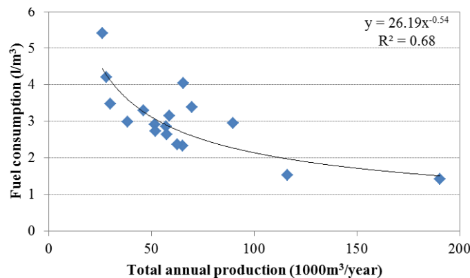
Figure 4. Relationships between fuel consumption and total annual production for GB systems
