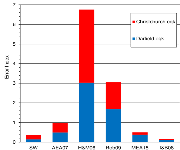
Figure 4. Average error indices across all case history sites. Lowest error indices between preferred and alternative critical layer interpretations shown.
