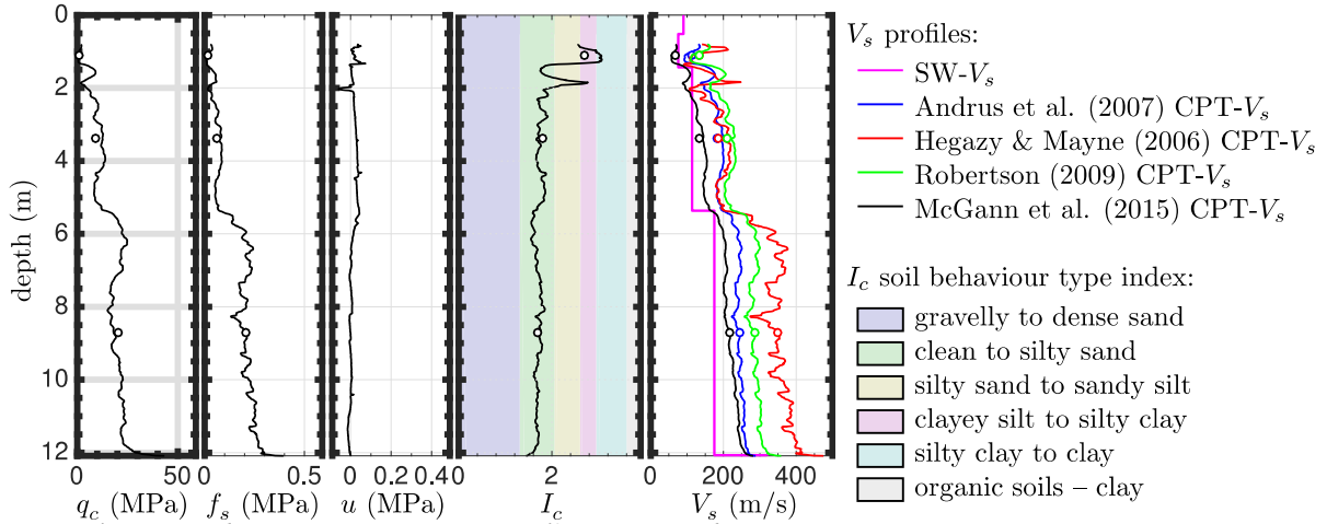
Figure 1. Comparison of SW- V_s and CPT- V_s profiles for a single site. CPT data and I_c profile provided for reference.
