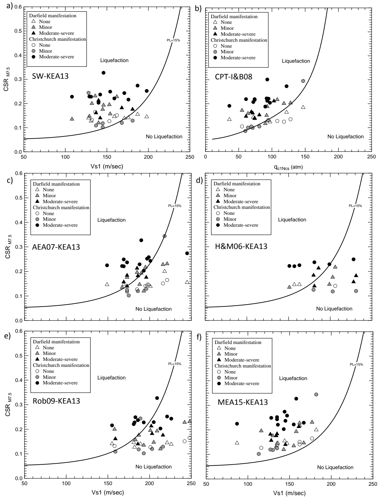
Figure 3. Liquefaction case history data plotted together with CRR_{M7.5} curves: a) Surface wave V_s data analyzed using KEA13, b) CPT q_{c1Ncs} data analyzed using I&B08, c) AEA07 V_s data analyzed using KEA13, d) H&M06 V_s data analyzed using KEA13, e) Rob09 V_s data analyzed using KEA13, f) MEA15 V_s data analyzed using KEA13.
