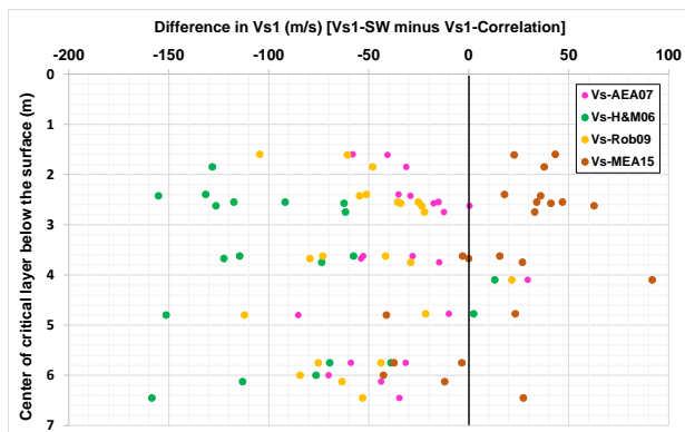
Figure 6. Difference in overburden-corrected shear wave velocity ( V_{s1} ) within the critical layer between SW- V_{s1} and CPT- V_{s1} as a function of depth to center of critical layer.
