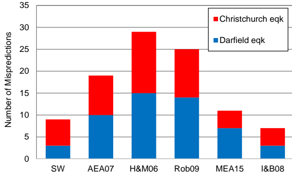
Figure 5. Number of incorrect case history predictions across all case history sites. Values are the lowest between preferred and alternative critical layer interpretations.
