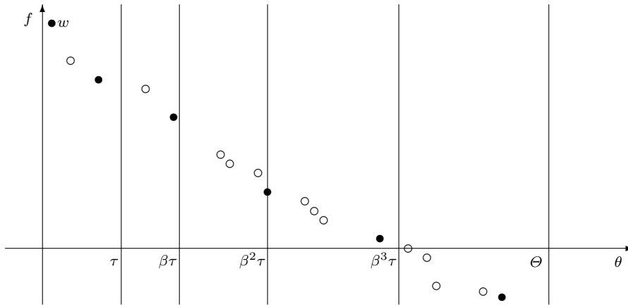
Fig. 2 This figure shows points in a filter before (circles and dots), and after pruning (dots only). The filter does not contain a feasible point. Pruning marks, as given in equation (9), are shown as vertical lines at \mu = \beta^j \tau where \tau is the tolerance on constraint violations, and \beta is the scale factor between adjacent marks. Here J_{\min} = 0 so the lowest positive mark is \mu = \tau . The marks do not extend beyond \Theta . The least infeasible point, marked w , is always included in the pruned filter. The remaining pruned filter points each minimize f over the set of filter points with constraint violations \theta less than or equal to some pruning mark.
