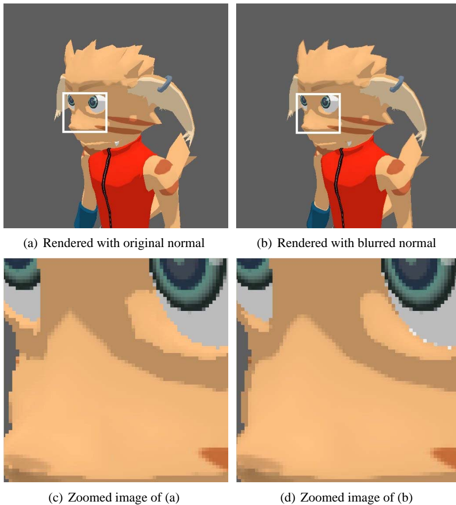
Figure 4.10: Shading comparison
