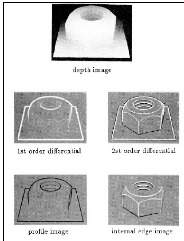
Figure 3.3: G-Buffer example [32]
