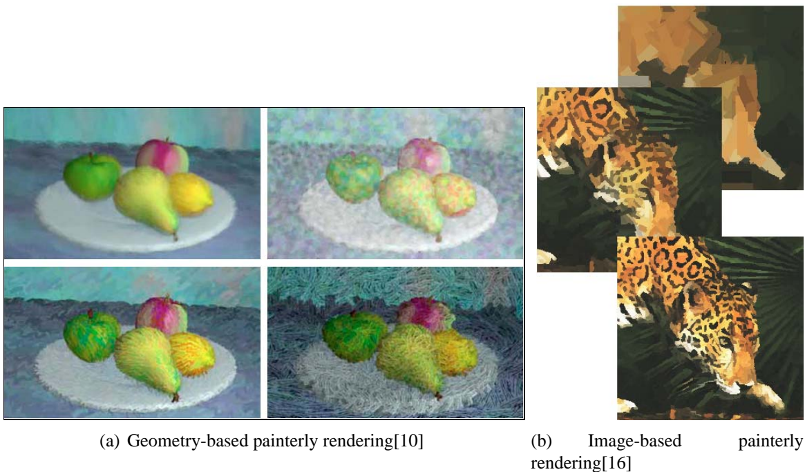
Figure 3.1: Painterly rendering
