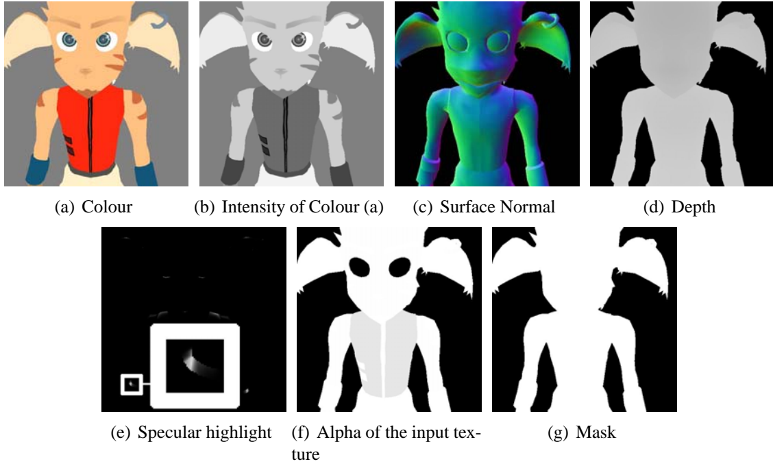
Figure 4.1: Rendered information
