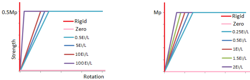
a) Splice strength of 50% of moment capacity
