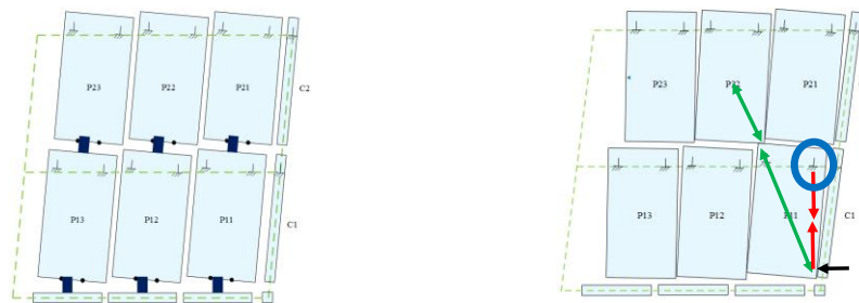
(a) Rocking Mode (with shear keys) (b) Typical Chinese Construction (without shear keys)
