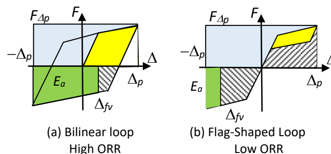
Figure 1. ORR for Different Hysteresis Loops
