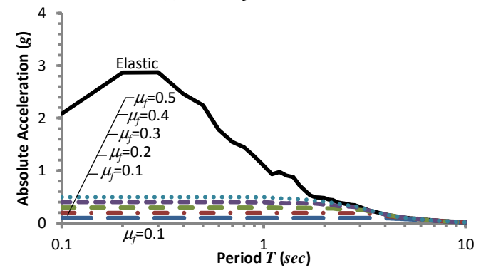
Fig. 4 Median response spectra
