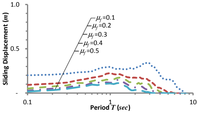
Fig. 5 Sliding displacement
