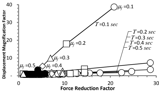
Fig. 8 Magnification and reduction factors relationships
