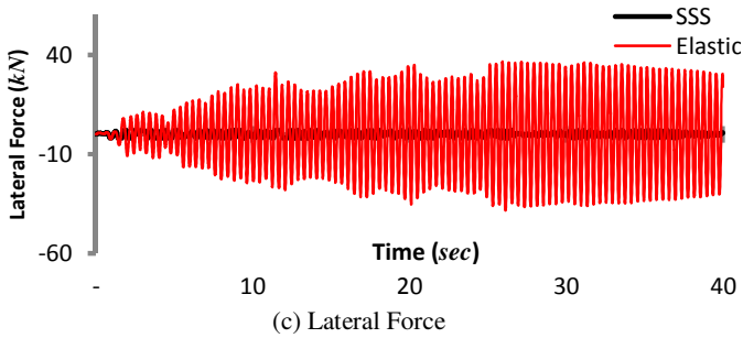
Fig. 2 Time history response ( T = 0.4 sec, \mu_f = 0.2 , LA01)
