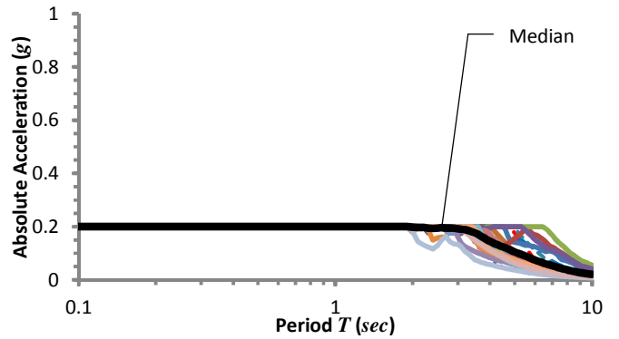
Fig. 3 Response spectra ( \mu_f = 0.2 , LA01)
