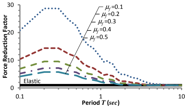
Fig. 7 Force reduction factor
