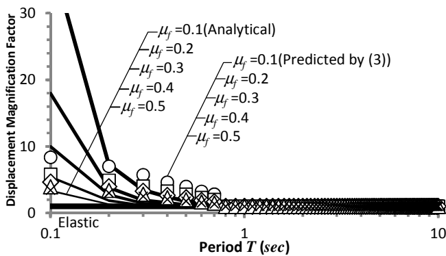
Fig. 9 Prediction of displacement magnification
