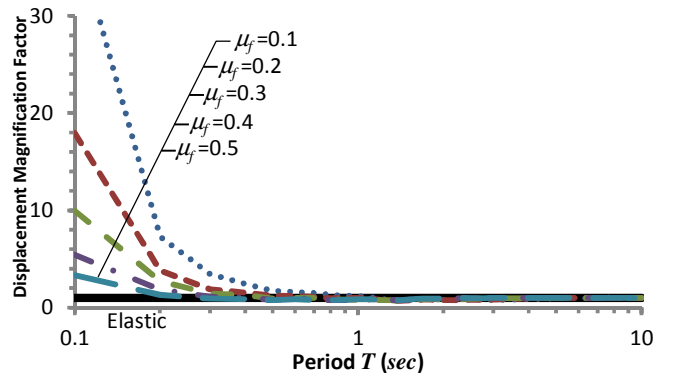
Fig. 6 Displacement magnification factor
