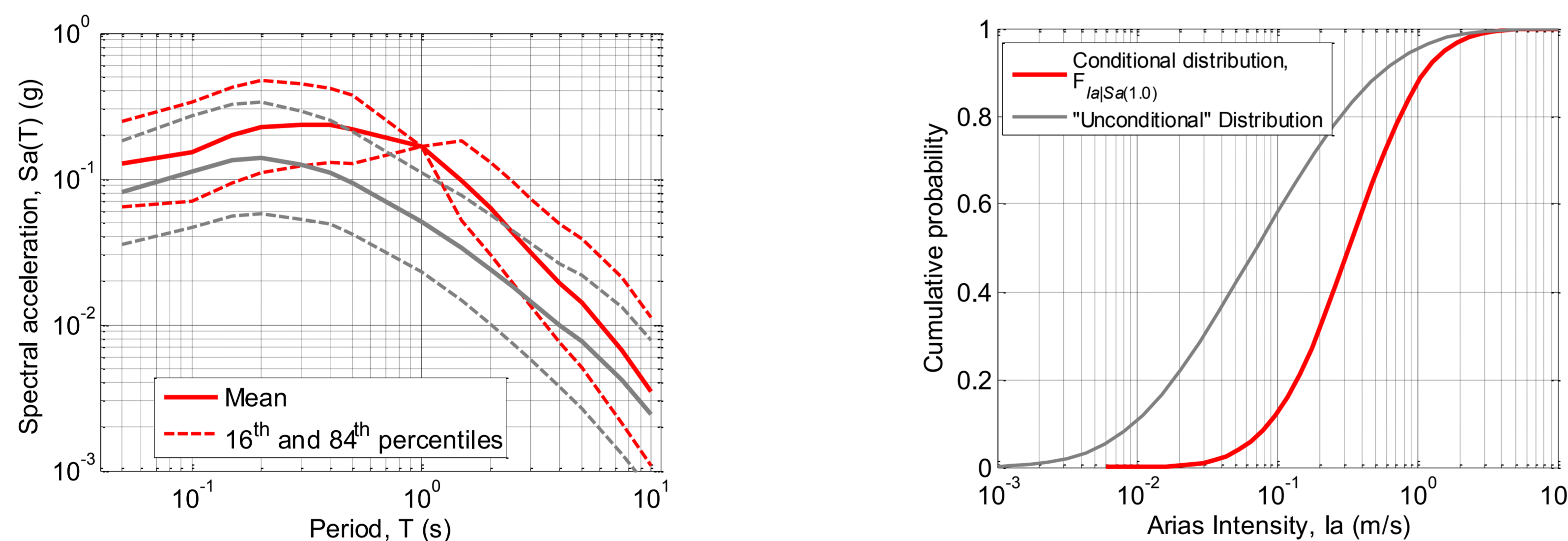
Figure 1: The disaggregation and example conditional distributions for a site in Christchurch, New Zealand.
