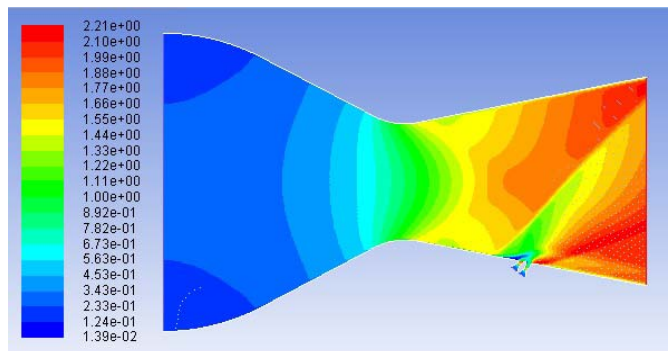
Fig. 5 The Mach number contour during vectoring using self-impinging supersonic secondary double jet with primary flow through a CD nozzle
