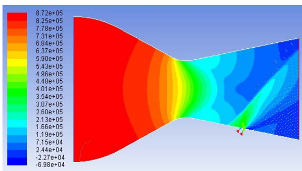
Fig. 7 The static pressure contour after vectoring using self-impinging supersonic secondary double jet with primary flow through a CD nozzle
