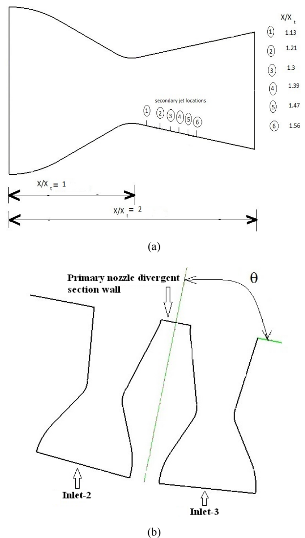
Fig. 1 Physical models of the primary and the self-impinging secondary nozzles: (a) Primary Nozzle ( A_e/A_t = 1.797 ) (b) Self-impinging secondary nozzles (enlarged view)
