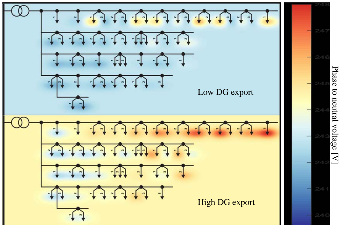
Figure 2 Examples of voltage effects caused by DG power export on a LV network, illustrated by colouring at the points of supply. For the low DG export case, 10% of ICPs are exporting and the network is load dominated. In the high DG export case 100% of ICPs are exporting and significant reverse power flow is occurring causing point of supply over-voltages at the downstream ends of feeders. The background colouring reflects the average network voltage.
