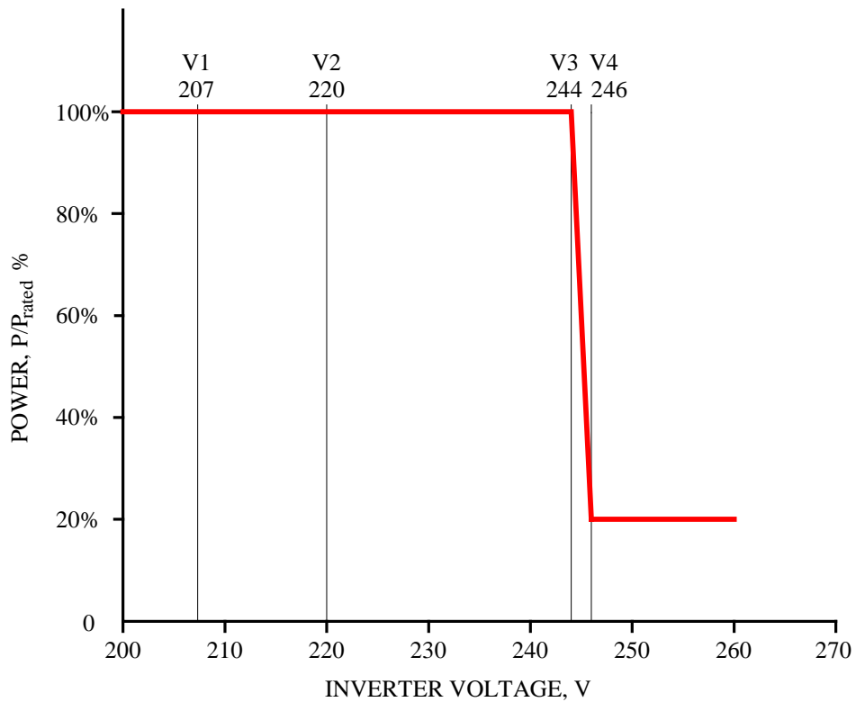
Figure 5 Curve for New Zealand Volt-Watt response mode.
