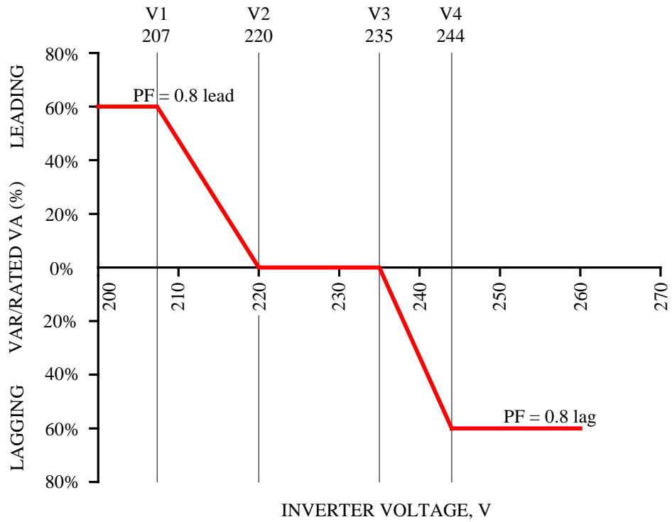
Figure 4 Curve for New Zealand Volt-VAr response mode.
