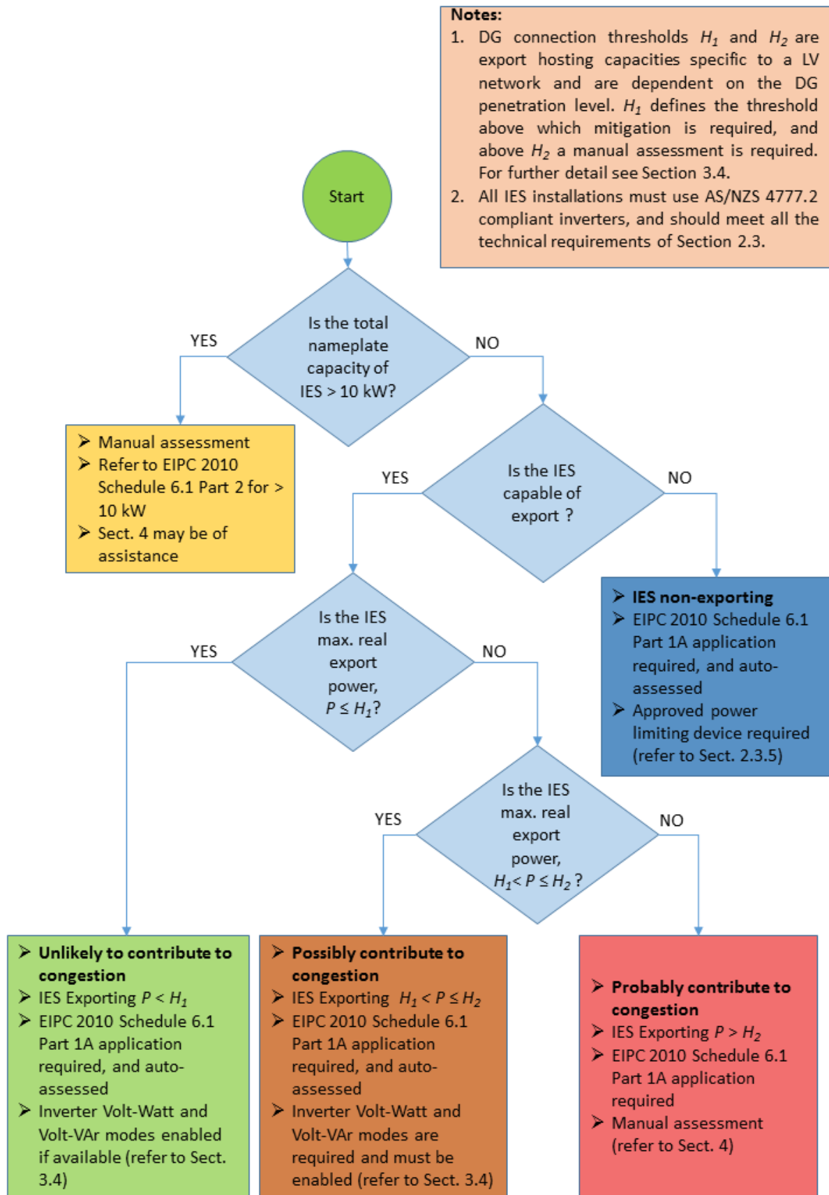
Figure 3 DG Guideline process flow diagram for assessing connection applications. Note that the diagram refers to sections in the Guideline.
