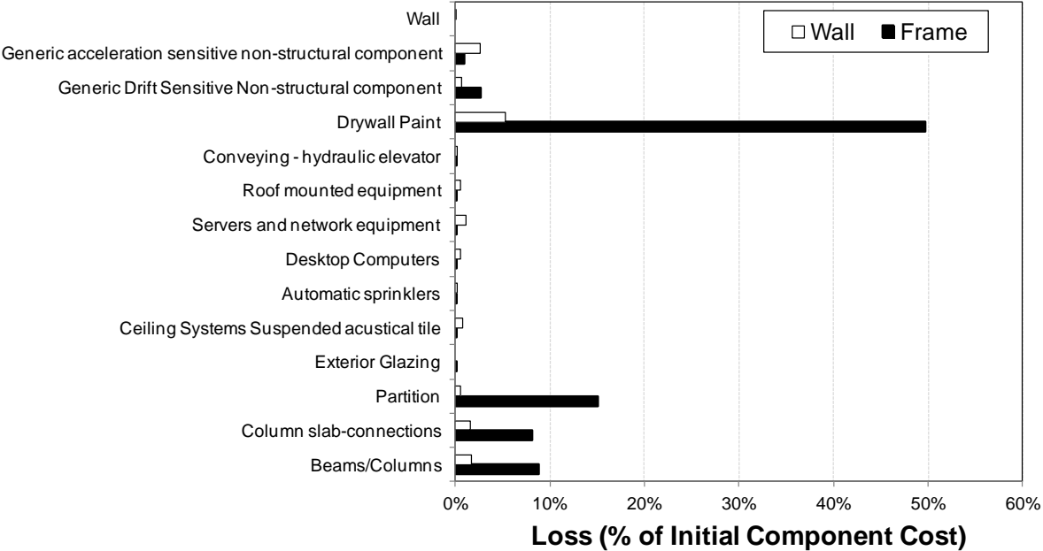
(a) 4 th of September 2010 scenario
