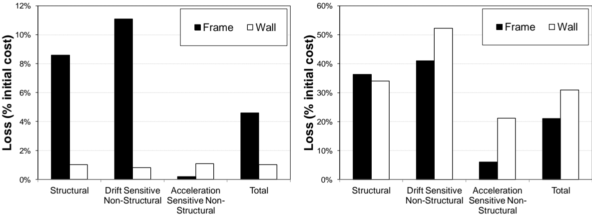
(a) 4 th September 2010 scenario (b) 22 nd February 2011 scenario Figure 5.4 Loss for each component group (percentage of component group’s initial cost)
