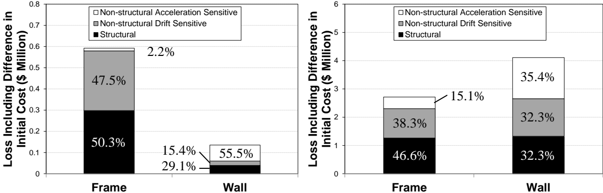
(a) 4 th September 2010 scenario (b) 22 nd February 2011 scenario Figure 5.5 Overall cost comparison (difference in initial cost and seismic losses)
