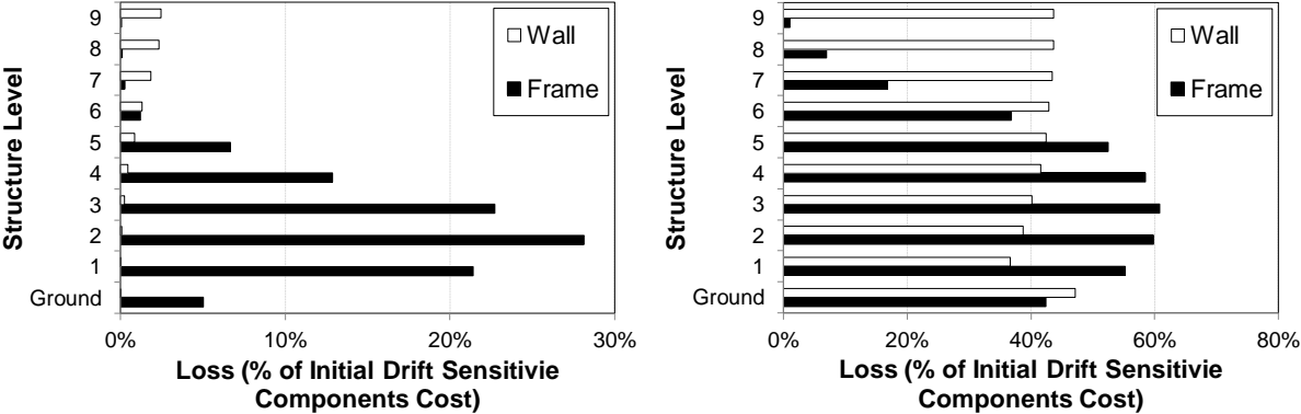
(a) 4 th September 2010 scenario (b) 22 nd February 2011 scenario Figure 5.1 Distribution of drift induced losses (structure and non-structural) for each storey level
