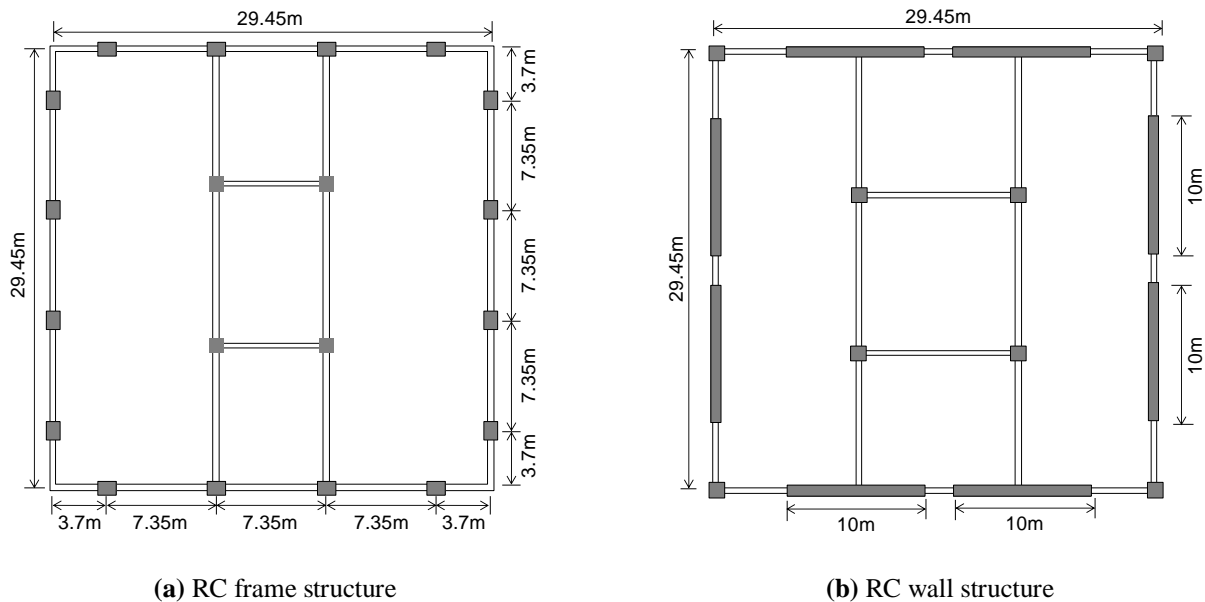
Figure 3.1 Plan elevations of RC structures considered in case study
