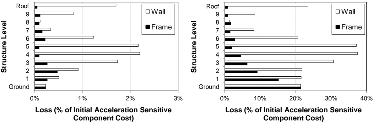
(a) 4 th September 2010 scenario (b) 22 nd February 2011 scenario Figure 5.2 Distribution of acceleration induced losses for each storey level
