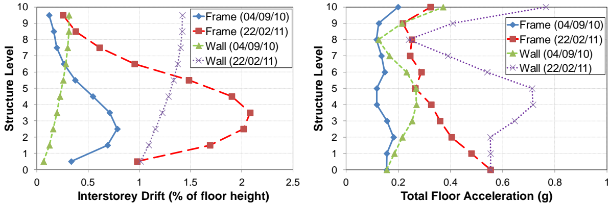
(a) Maximum Inter-storey Drift Profiles
