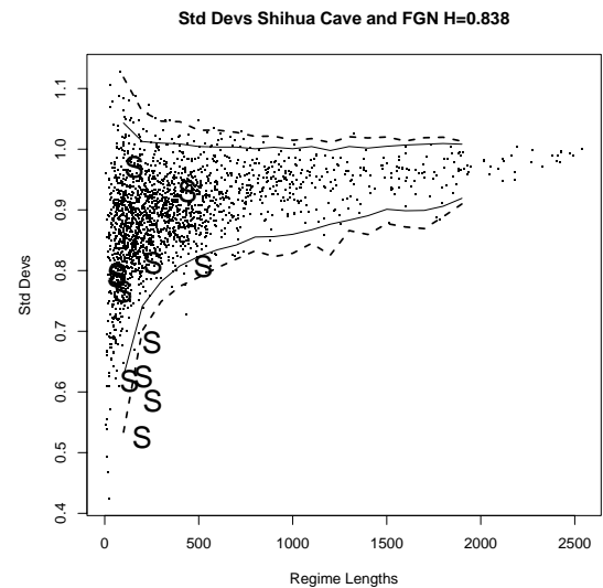
Figure 7. Estimates of regime standard deviations for Shihua Cave temperature reconstruction and simulated FGNs with H=0.838 .
