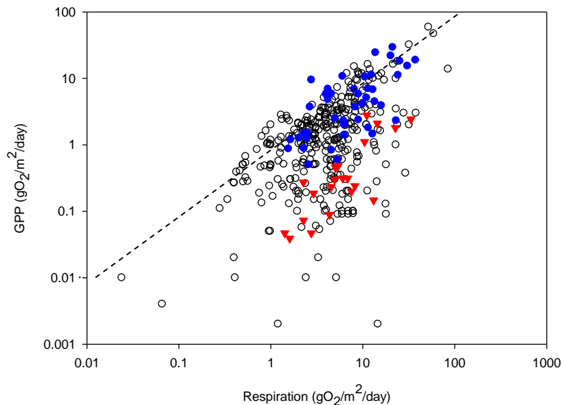
Figure 2. In-stream primary production (GPP) and respiration for 21 streams from the Canterbury region (New Zealand) relative to measurements from other New Zealand studies and international studies. Red triangles represent production and respiration at individual sites across Canterbury, blue dots represent primary production and respiration measurements in other New Zealand studies, and black circles represent measurements made internationally. The dashed line represents a production to respiration ratio of one.
