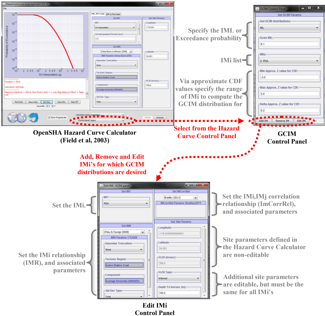
Figure 2: The OpenSHA hazard curve calculator and the GCIM control panels
