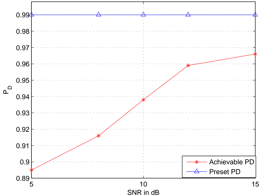
Figure 4.26 Performance degradation for the truncated sequential detector for a log-normal shadowing channel at different received SNR ( \sigma_{dB} = 6dB ).
