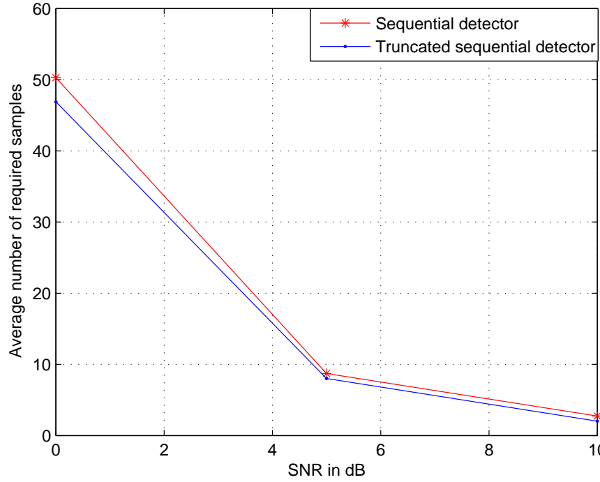
Figure 4.19 Average number of required samples for the truncated sequential detector for a AWGN channel at different received SNR.
