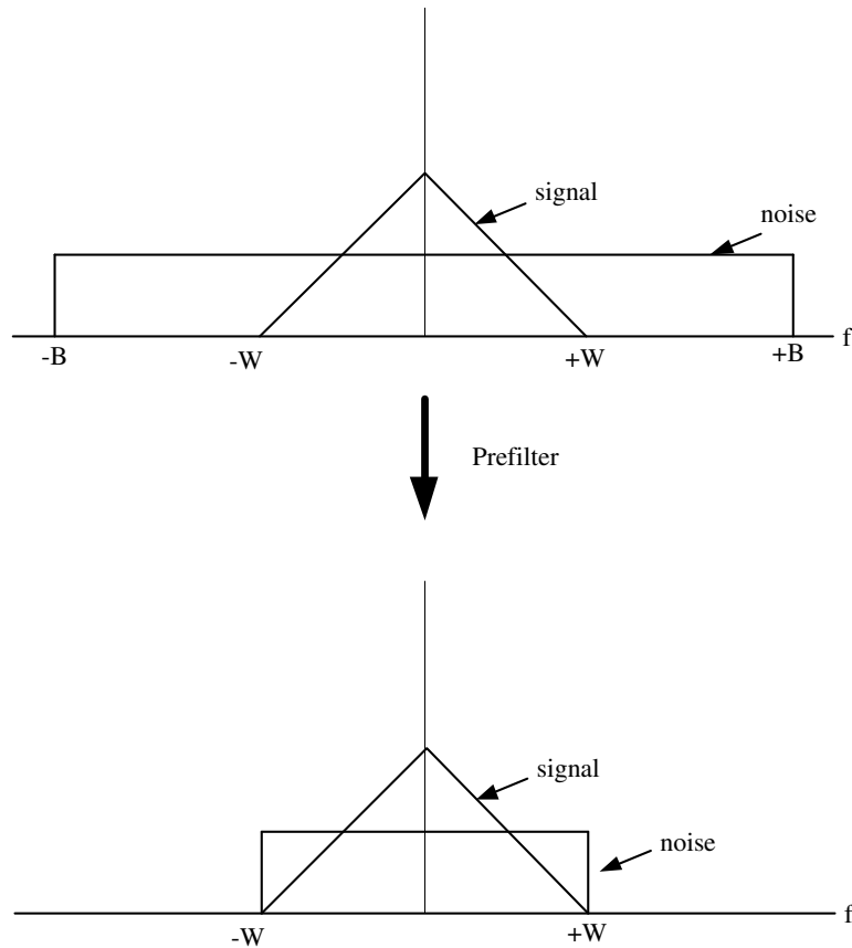
Figure 3.4 Narrowband detection.
