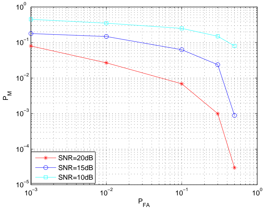
Figure 4.5 Complementary ROC curves for a log-normal shadowing channel at different average SNR (10 samples per block).
