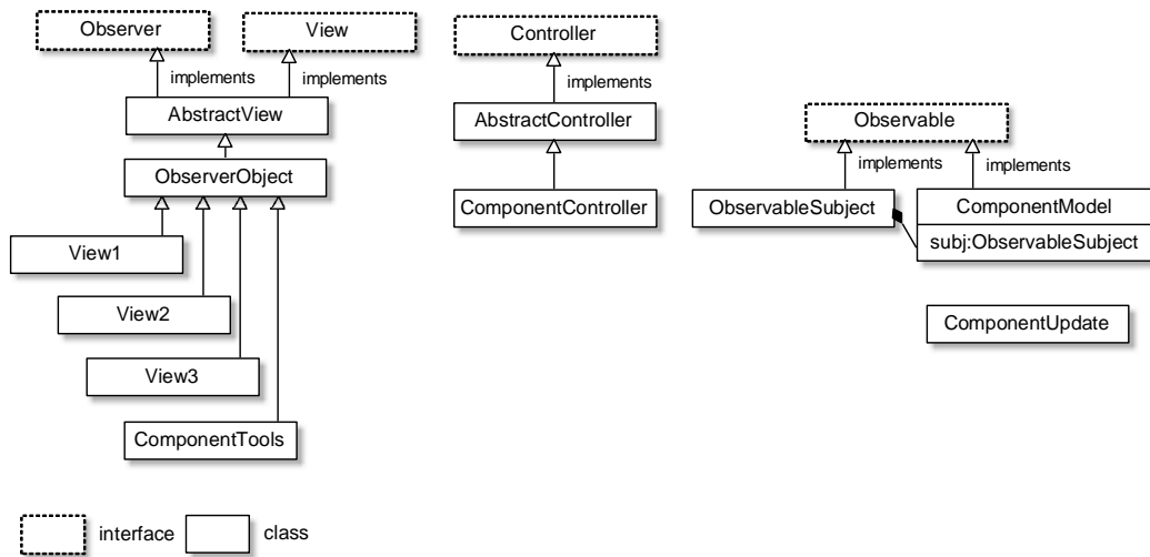
Figure 5.4 The DES MVC Structure
