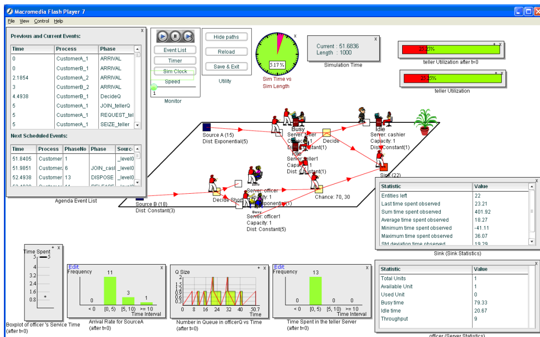
Figure 5.8 A Final Model
