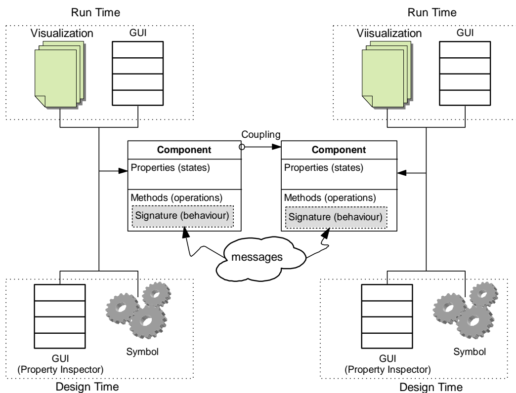
Figure 4.5 Component Architecture
