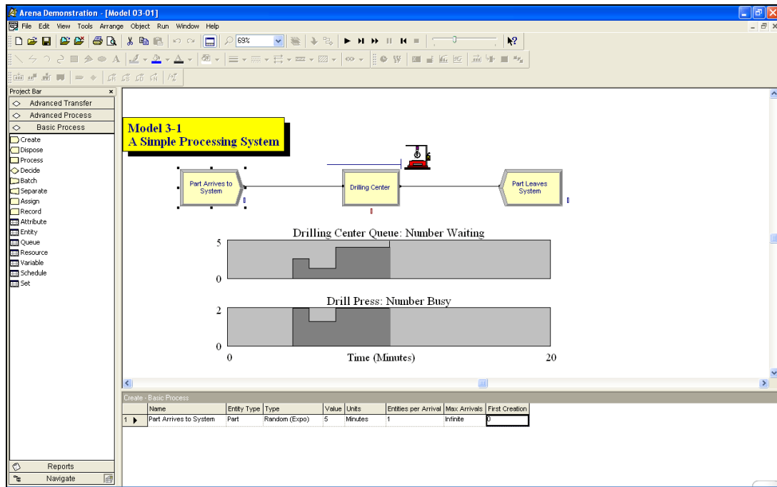
Figure 6.4 Arena Screenshot
