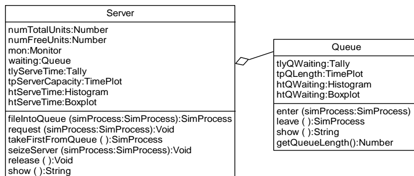
Figure 3.7 Class Diagram for the Resource Package
