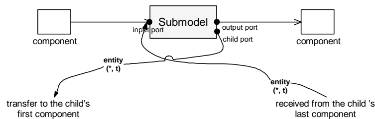
Figure 5.11 Submodel Architecture and Transferring Mechanisms
