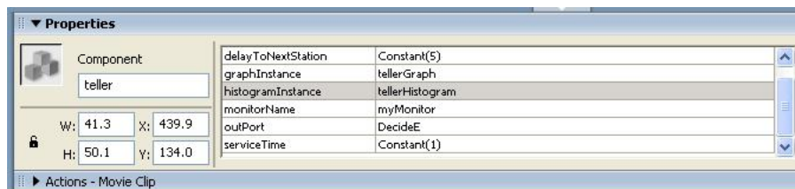
Figure 5.7 A Server's Properties and Default Values
