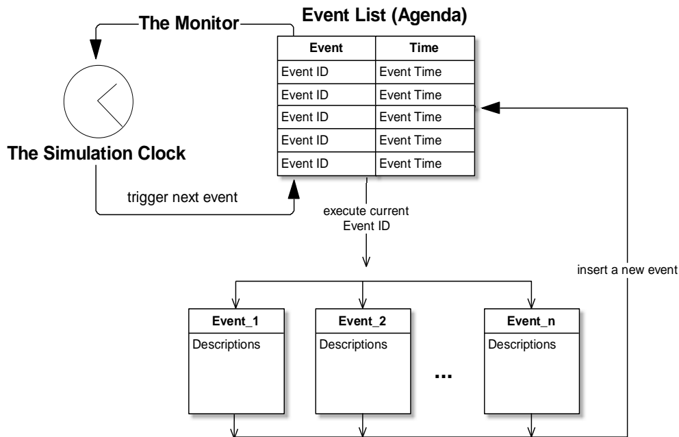
Figure 3.1 The Event-Oriented Approach Mechanism
