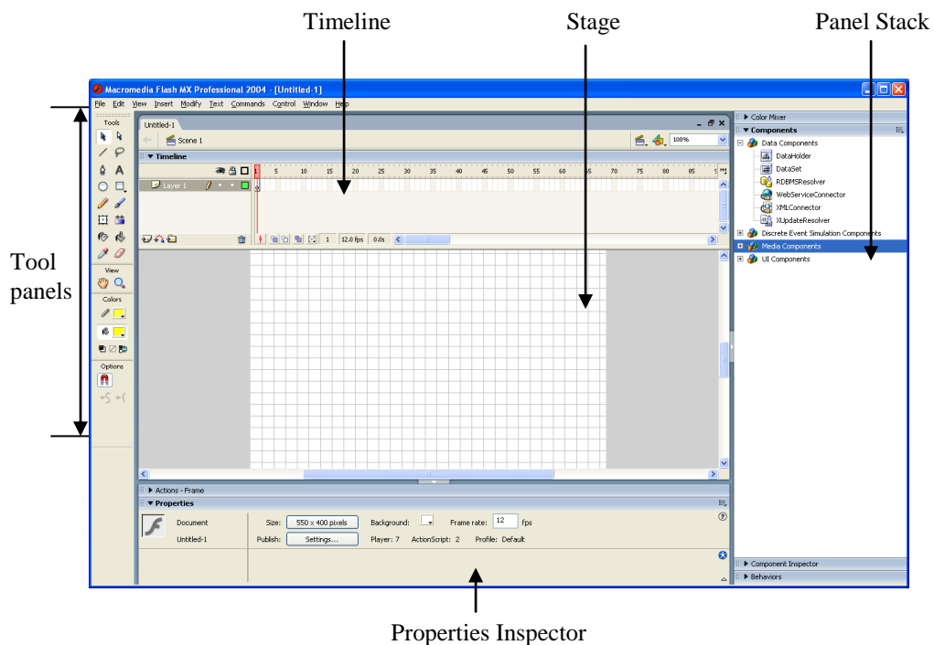
Figure 2 The Flash's Development Environment
