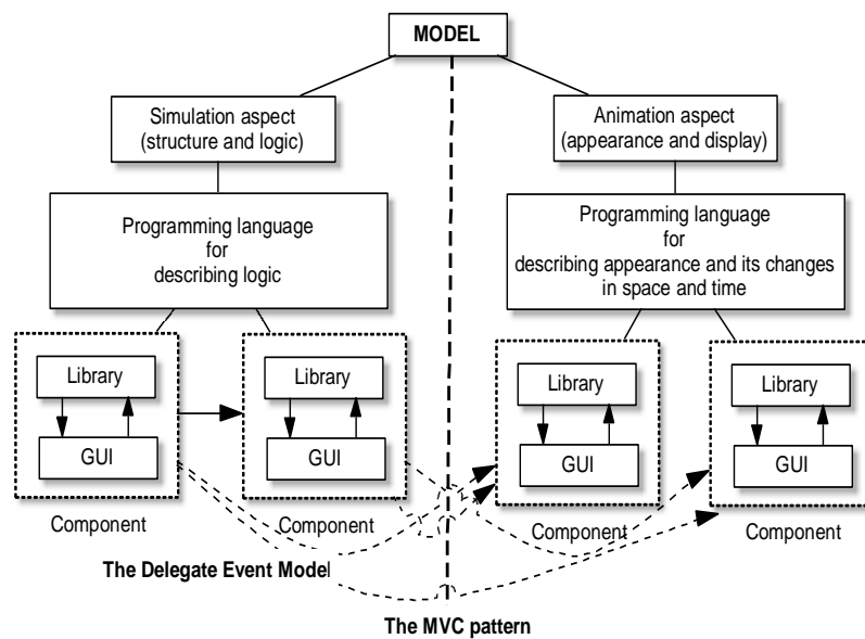
Figure 5.1 Simulation and Animation Aspects of a Model
