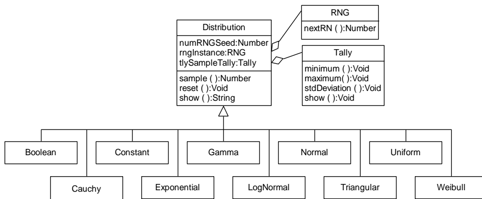
Figure 3.5 Class Diagram for the Distribution Package
