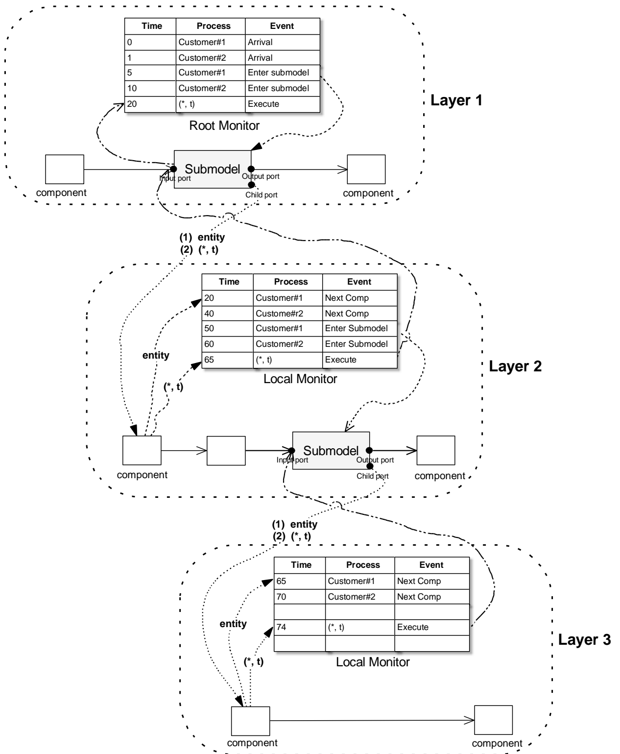
Figure 5.12 Monitor Delegation Mechanism
