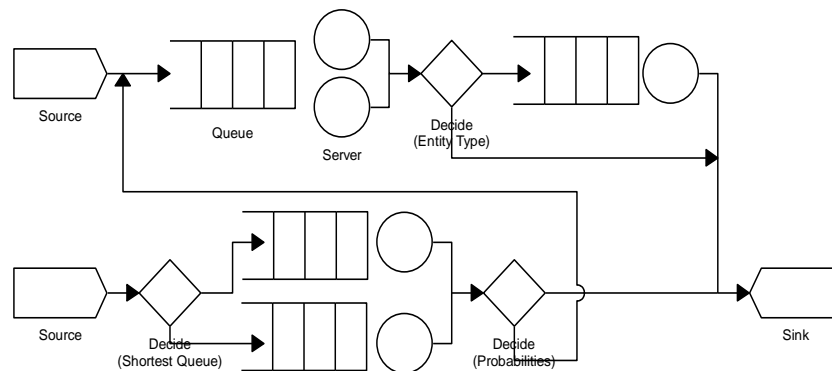
Figure 5.6 A Queuing Network System
