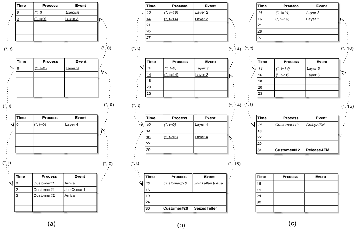
Figure 5.15 Agenda States
