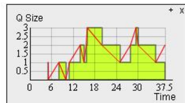
Number in Queue in officerQ vs Time (after t=5)
