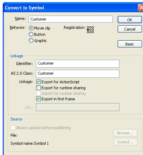
Figure 7 Associating a Movie Clip Symbol with Its Relevant Class
