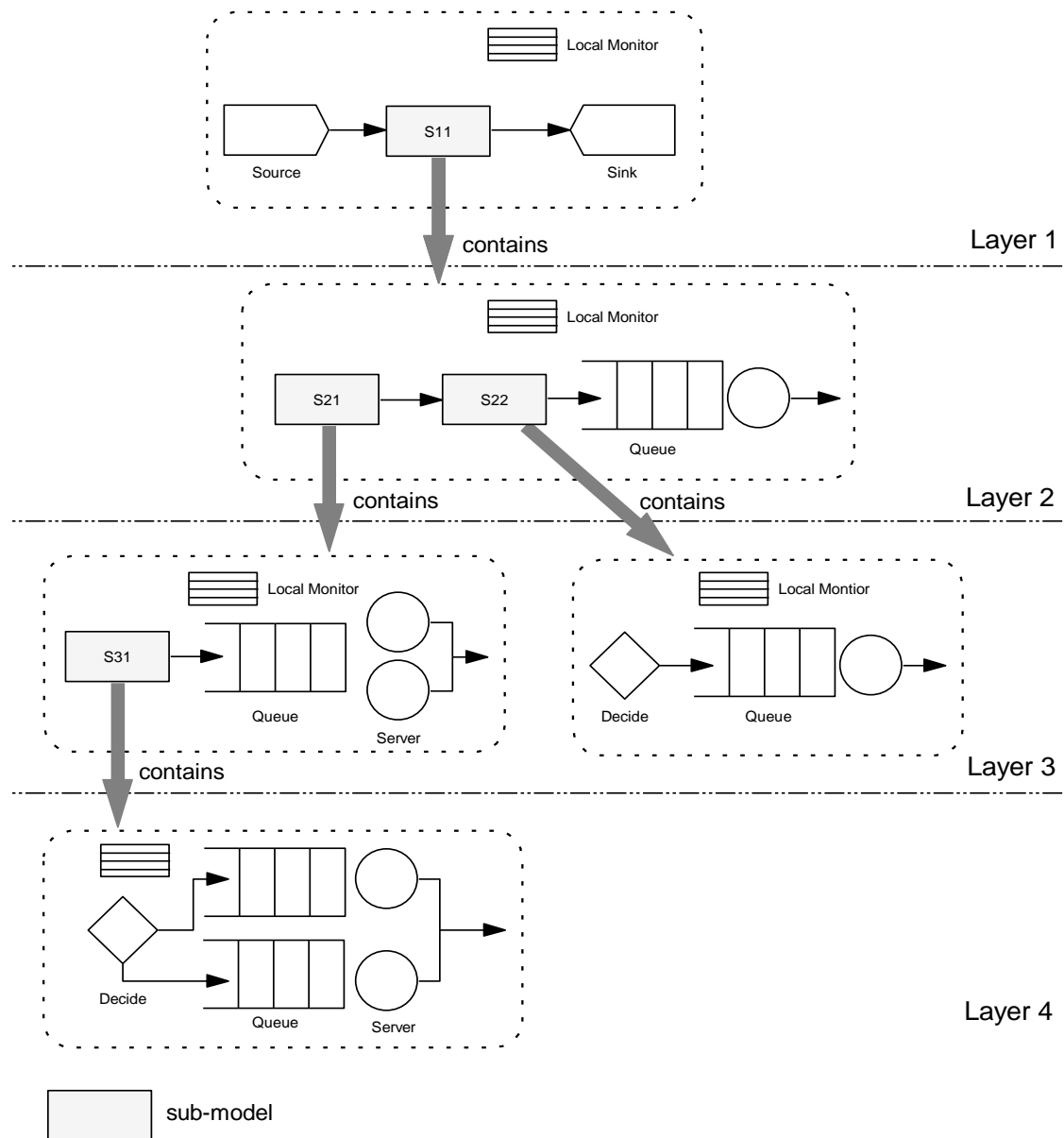
Figure 5.10 Hierarchical Construction of a DES Model
