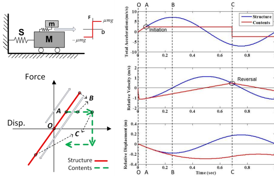
Figure 3.1 Response history of structure-contents sliding system
