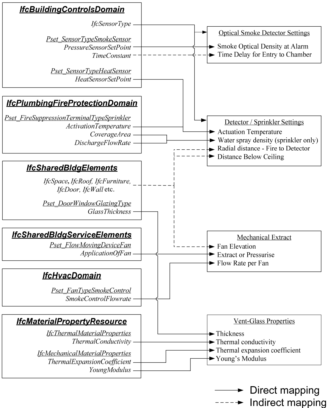
Figure 10. Summary of mapping from IFC 2x2 to BRANZFIRE.
