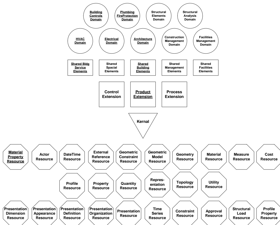
Figure 1. IFC 2x2 schema overview, adapted from ref. [14].
