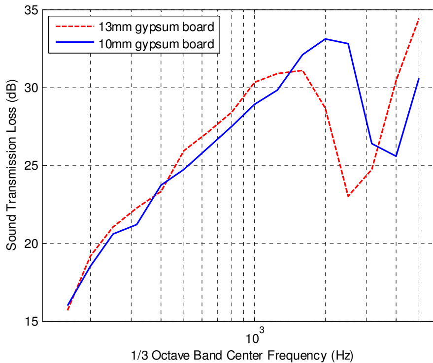
Figure 10 Cambridge’s results for the effect of the panel thickness on the sound transmission loss of a 10 and 13 mm single panel gypsum board
