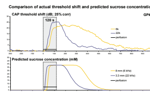
Figure 4: The difference between the CAP threshold time-courses at 6 kHz and 22 kHz was at least partially accounted for by the concentration of the sucrose at the scala tympani predicted by the Washington University Cochlear Fluids Simulator (v1.6h; Salt, 2002) at locations roughly corresponding to the 6 kHz and 22 kHz sites (assuming a 22 mm guinea-pig cochlea and the place-frequency map of Tsuji and Liberman, 1997).
