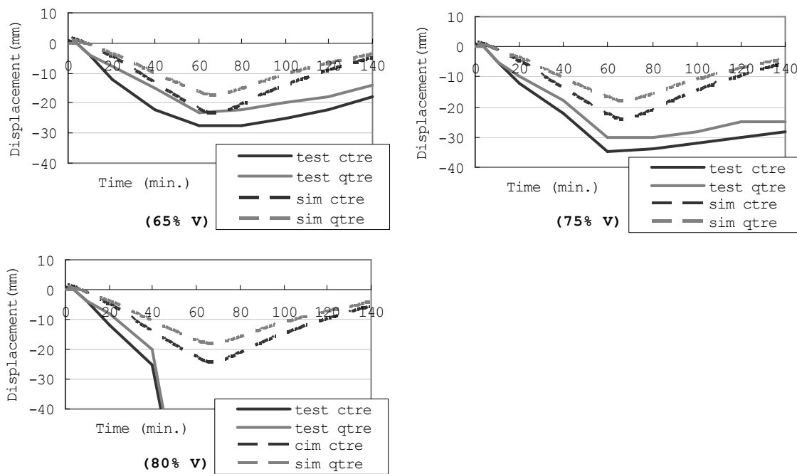
Fig. 8 – Comparison between the vertical displacements at midspan (ctre) or at the location of the point load (qtre) from simulation (sim) and test (test) results
