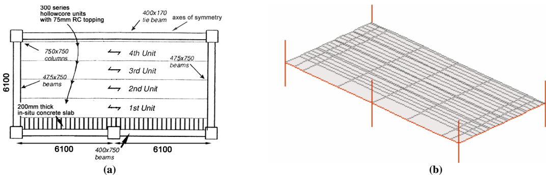
Fig. 9 – Half of the floor plan of simulated test (a) from the drawing 25 (b) in simulation
