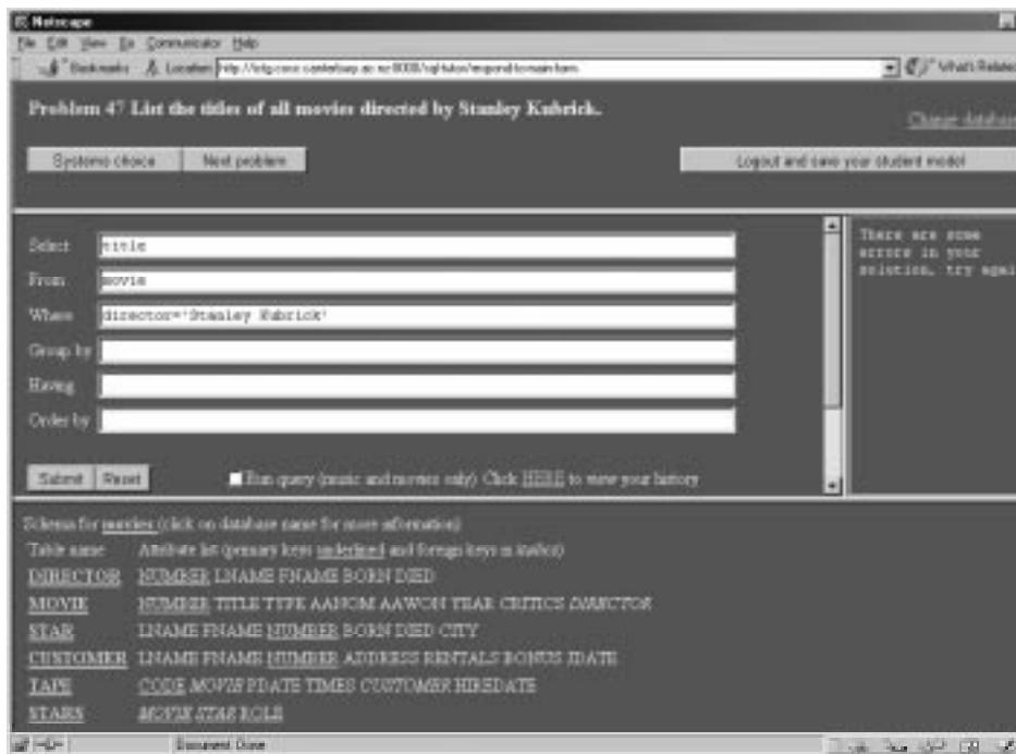
Fig. 2. Interface of the Web-enabled version of SQL-Tutor
