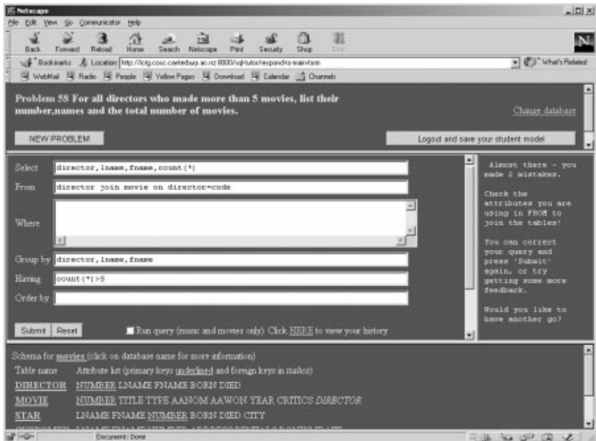
Fig. 6. Interface of the Web-enabled version of SQL-Tutor
