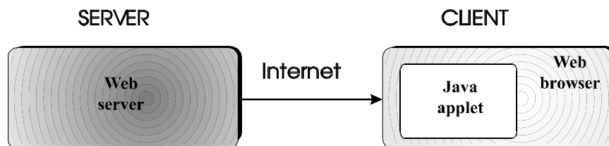
Fig. 2. Replicated architecture
