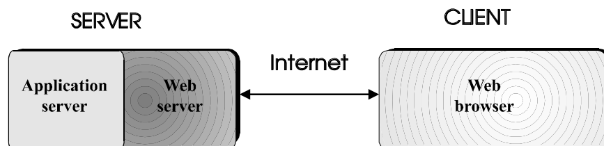
Fig. 1. Centralized architecture
