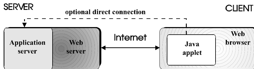
Fig. 3. Distributed architecture
