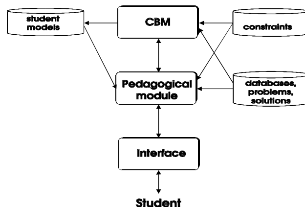
Fig. 4: Architecture of SQL-Tutor
