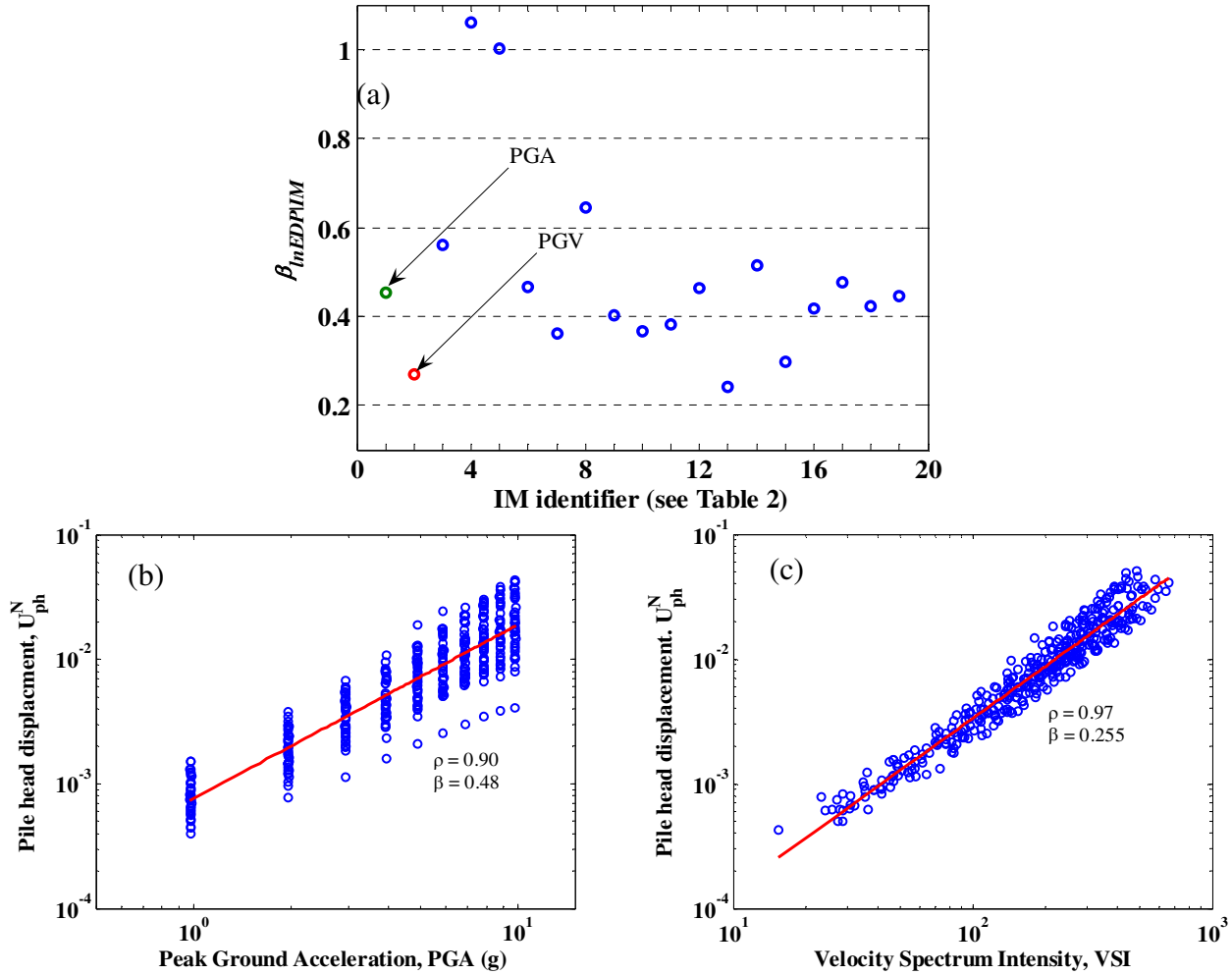
FIG. 3: Efficiency of the candidate IMs. (a) Efficiency of all IMs as a function of \beta_{inEDPIM} ; (b)&(c) EDP-IM scatter plots for PGA and VSI, respectively.
