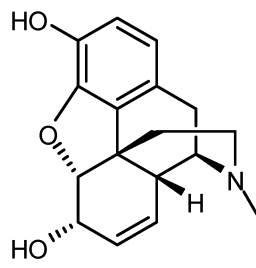
Morphine Advanced Synthesis & Catalysis
