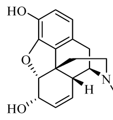
Morphine Journal of Molecular Modeling
