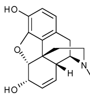
Morphine Royal Society of Chemistry publications
