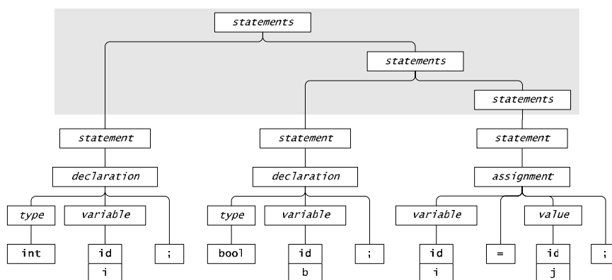
Figure 19: Example parse tree for recursive grammar
