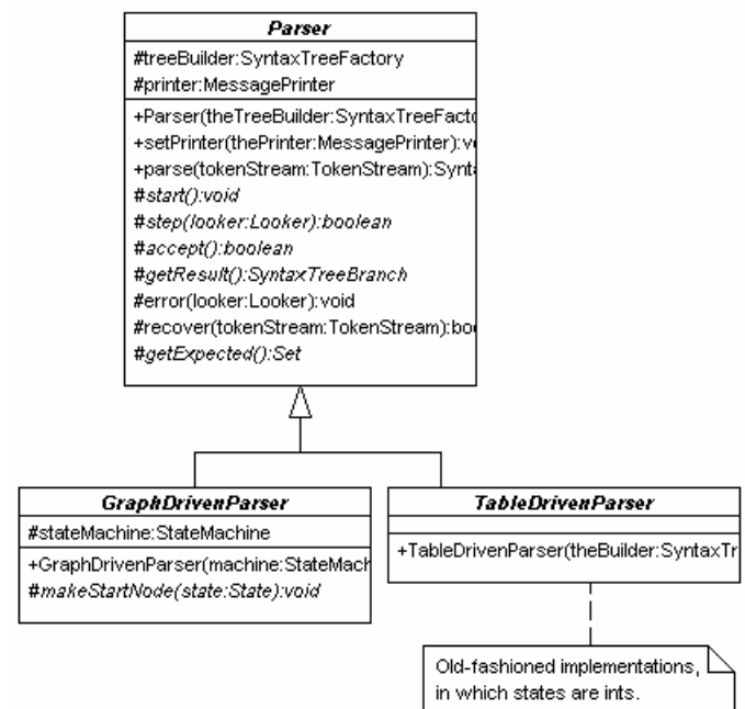
Figure 64: PDA base classes
