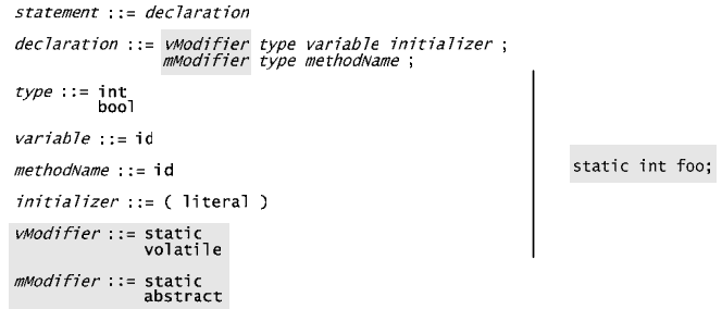
Figure 46: Grammar modified to require a GLR parser
