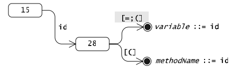
Figure 39: SLR(1) PDA fragment with inadequate state
