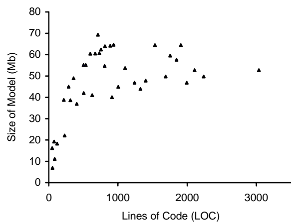
Figure 105: JST memory usage
