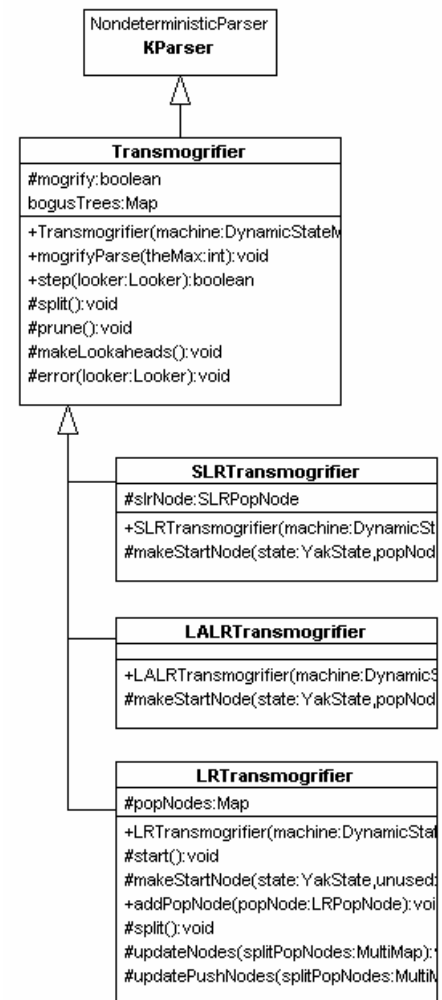
Figure 82: Transmogrifier classes
