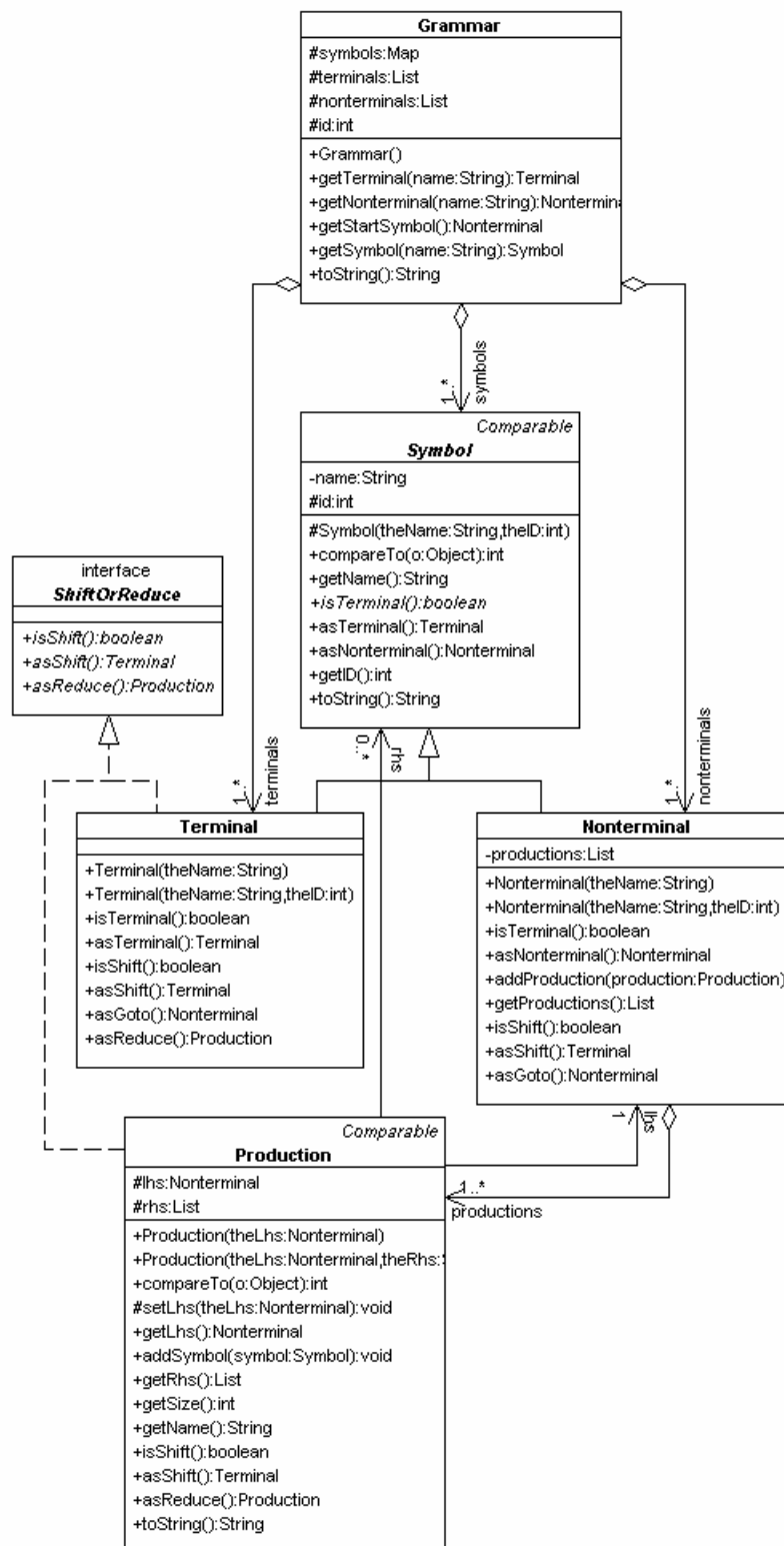
Figure 58: Grammar classes
