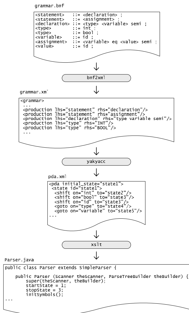
Figure 51: Decoupled architecture of yakyacc
